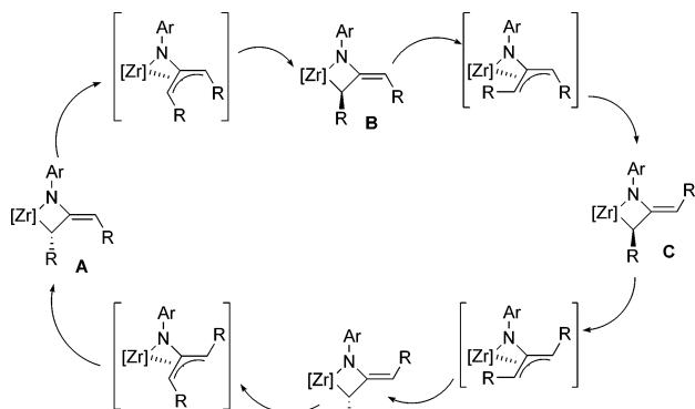
Figure 7. [1,3]-Shift mechanism for E/Z isomerization and racemization.
