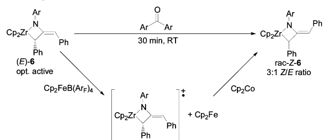
Scheme 9. Insertion Reactions of Diphenylmetallacycle 6
