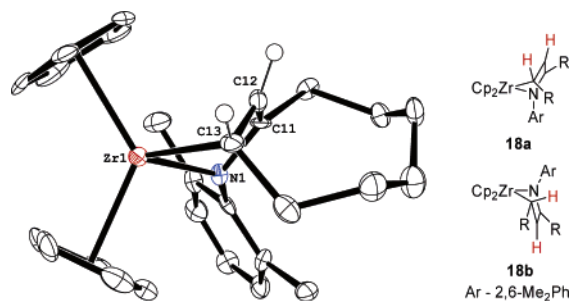
Figure 3. X-ray structure of MAD complex 18a . 50% probability boundaries are indicated. Bond distances: Zr1–N1 2.160 Å, Zr1–C13 2.254 Å, Zr1–C11 2.652 Å, Zr1–C12 2.497 Å, N1–C11 1.385 Å, C11–C12 1.386 Å, C12–C13 1.441 Å. Bond angles: N1–Zr1–C13 83.7°.
