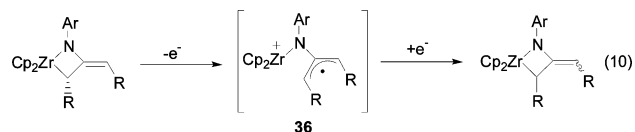
Figure 7. [1,3]-Shift mechanism for E/Z isomerization and racemization.
