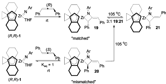
Scheme 6. Formation of Matched and Mismatched Metallacycles and Establishment of the Equilibrium Mixture
